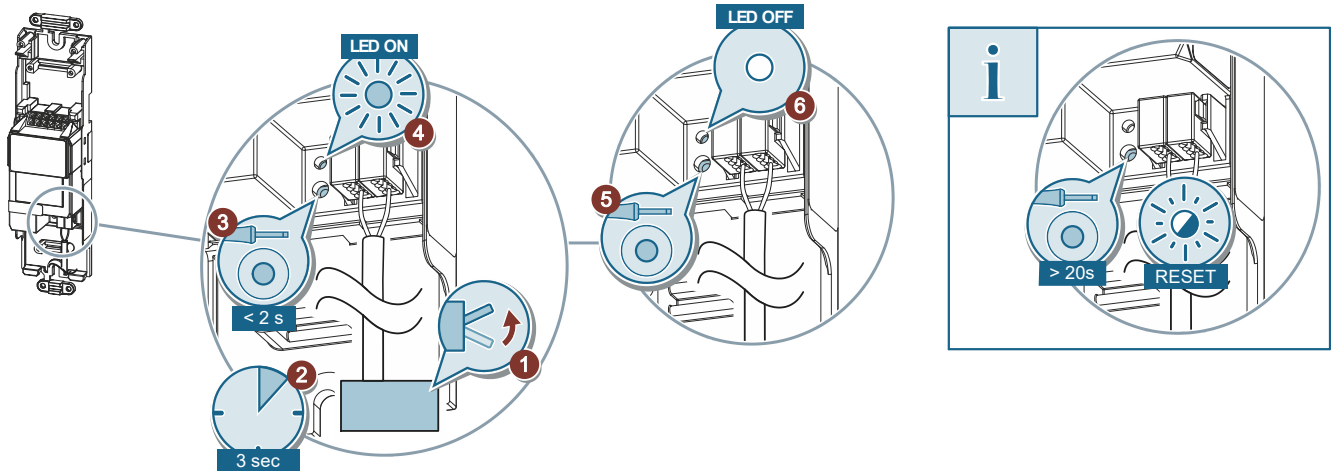
Fig. 5: KNX test
