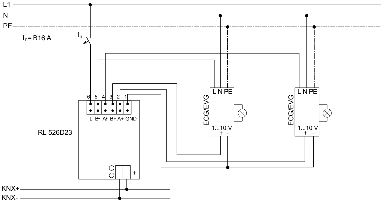
Fig. 6: Connection example
